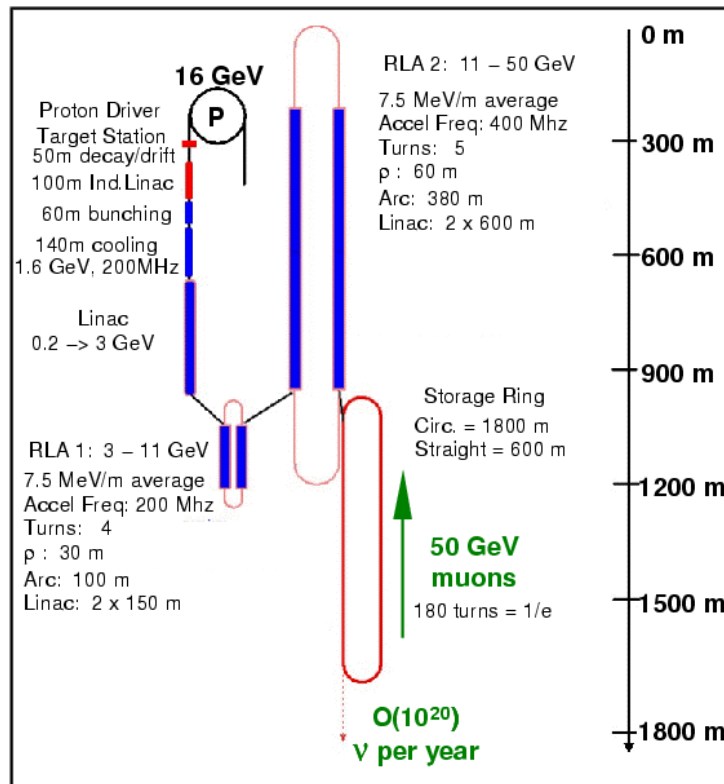
Figure 5.3. A Neutrino Factory. A muon-based neutrino factory is another long-term option for the field. Such a facility might lead to a high-energy muon collider.
