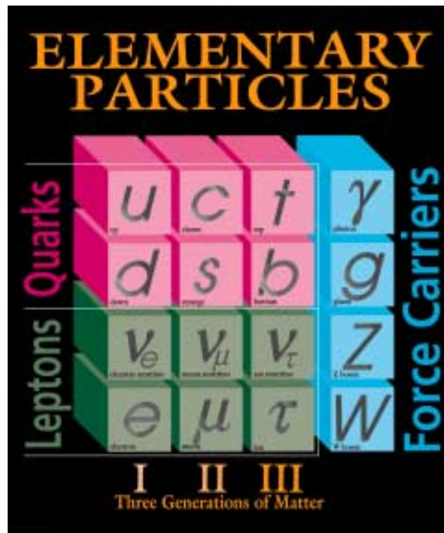
Figure 1.2. The Standard Model of Particle Physics. The six quarks and six leptons interact through the strong, weak and electromagnetic forces. The forces themselves are described by particles, labeled \gamma , g, W and Z.
