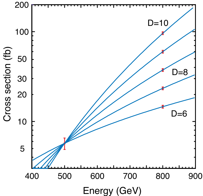
Figure 3.4. Extra Dimensions. The linear collider can measure the number (D) of space-time dimensions, using events in which particles disappear into the extra dimensions. From Wilson, LC-PHSM-2001-010.
