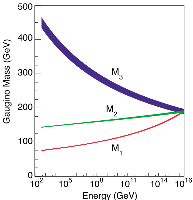
Figure 3.3. Quantum Dimensions. Discovery of gaugino mass unification requires precision measurements from the LHC ( M_3 ) and the linear collider ( M_1 and M_2 ). From Blair, Porod and Zerwas, hep-ph/0007107.
