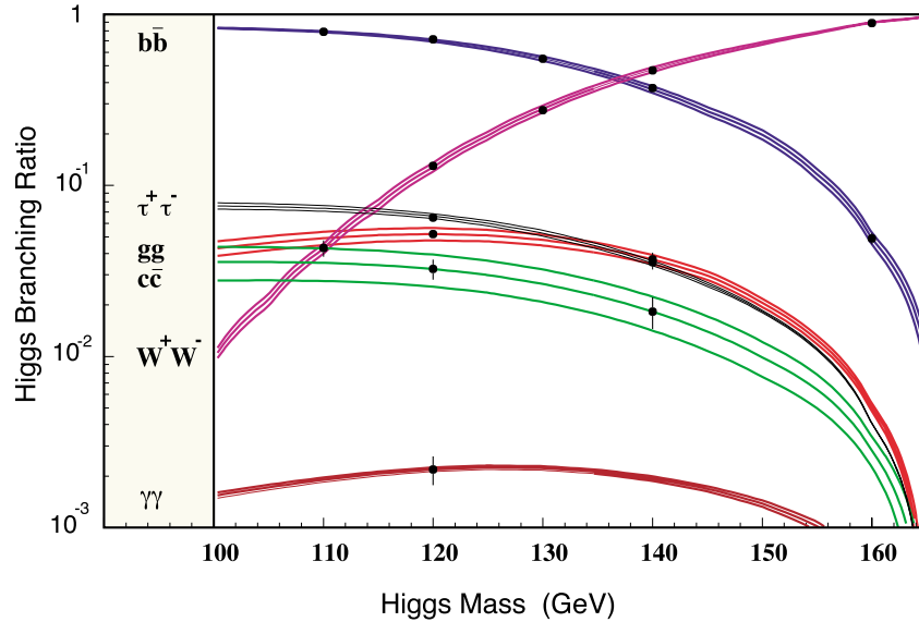
Figure 3.2. Decays of the Higgs. A high-luminosity linear collider can measure Higgs boson couplings to see whether the Higgs particle is responsible for the origin of mass. From Battaglia, hep-ph/9910271.
