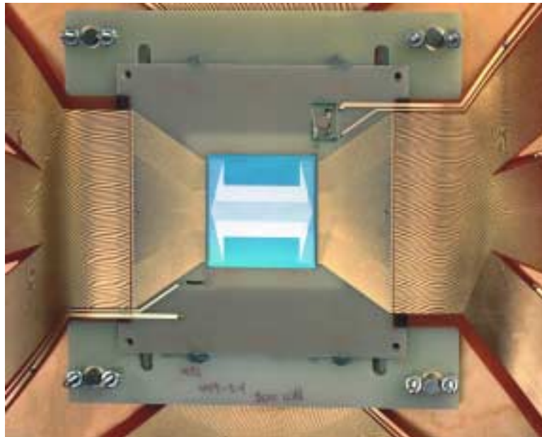
Figure 5.4. Detector R&D. Particle physics detectors challenge the state-of-the-art in electronics and other technologies.
