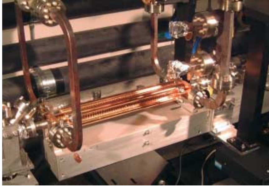
Figure 4.2. Linear Collider R&D. The photo shows a test accelerating structure for the NLC.
